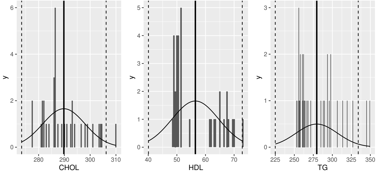
Figure 1: Discrete histogram and the corresponding normal distribution.
