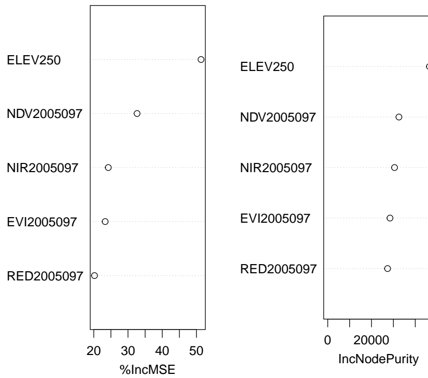
Figure 2: Example 1 - Variable importance graph for Sage percent cover (RF model).
