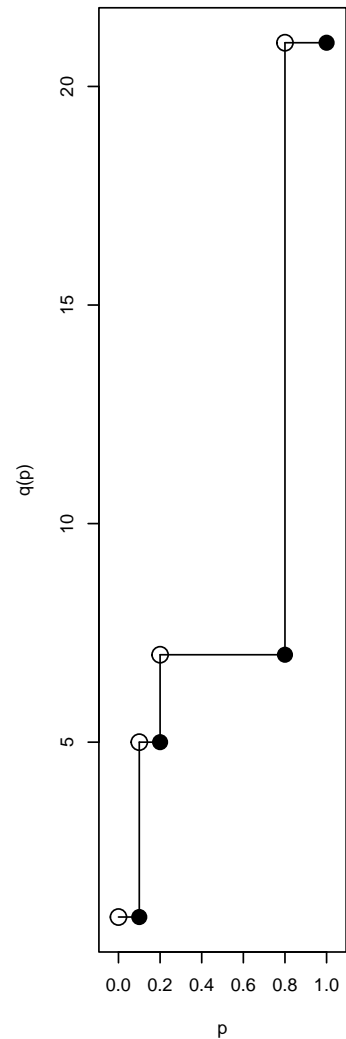
Quantile function of DiscreteDistribut
