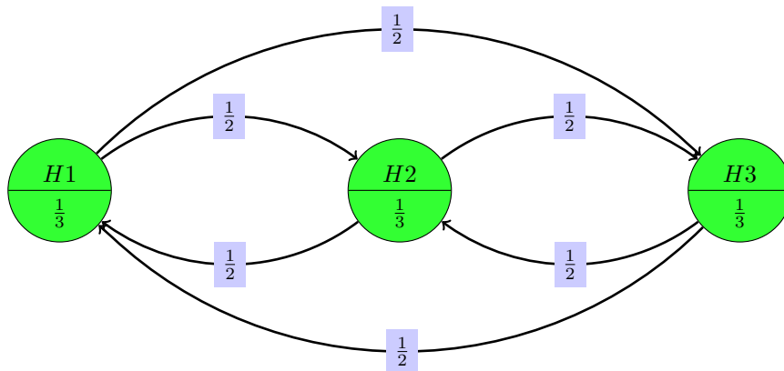
Figure 1.1: Graph representing the Bonferroni-Holm-Procedure for three hypotheses.
