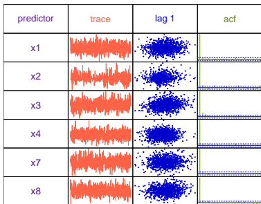
Figure 4: The graphic produced by the command checkChains(fit3) for the ganselBayes() fit object fit3 . The Figure 1 caption provides full details on checkChain() graphics.
