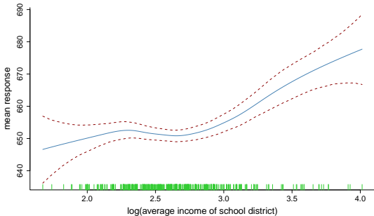
Figure 14: The plots produced from the command plot(fit13,shade = FALSE,estCol = "steelblue",varBandCol = "darkred", rugCol = "limegreen",xlab = "log(average income of school district)",cex.lab = 1.75) for the gamselBayes() fit, stored as fit13 . The shaded regions correspond to pairwise 95% credible intervals. The rug at the base of the plot show values of each predictor.
