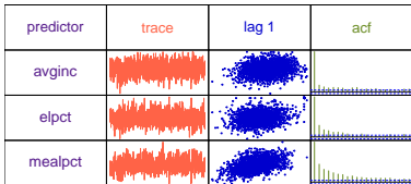
Figure 6: The graphic produced by the command checkChains(fit5) for the ganselBayes() fit object fit5 . The Figure 1 caption provides full details on checkChain() graphics.
