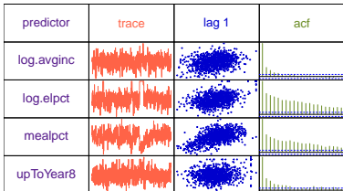
Figure 8: The graphic produced by the command checkChains(fit6) for the ganselBayes() fit object fit6 . The Figure 1 caption provides full details on checkChain() graphics.
