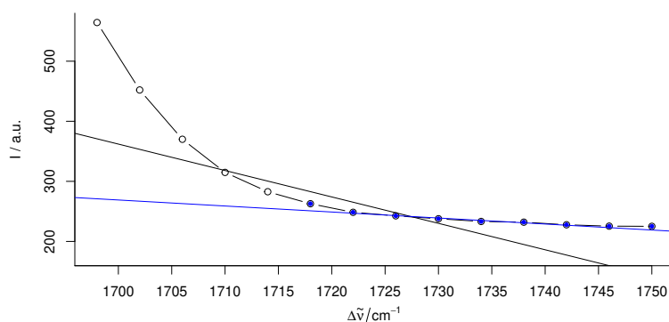
Figure 3 Influence of fit.to on the baseline polynomial. The black baseline is fit to the spectral range 1700\text{--}1750\text{ cm}^{-1} , the blue to 1720\text{--}1750\text{ cm}^{-1} only.
