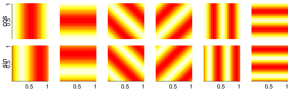
Figure 2: Illustration of two dimensional Fourier basis functions used in the discrete real Fourier transform. On the x- and y-axis are the coordinates of \mathbf{s} = (s_x, s_y)' .
